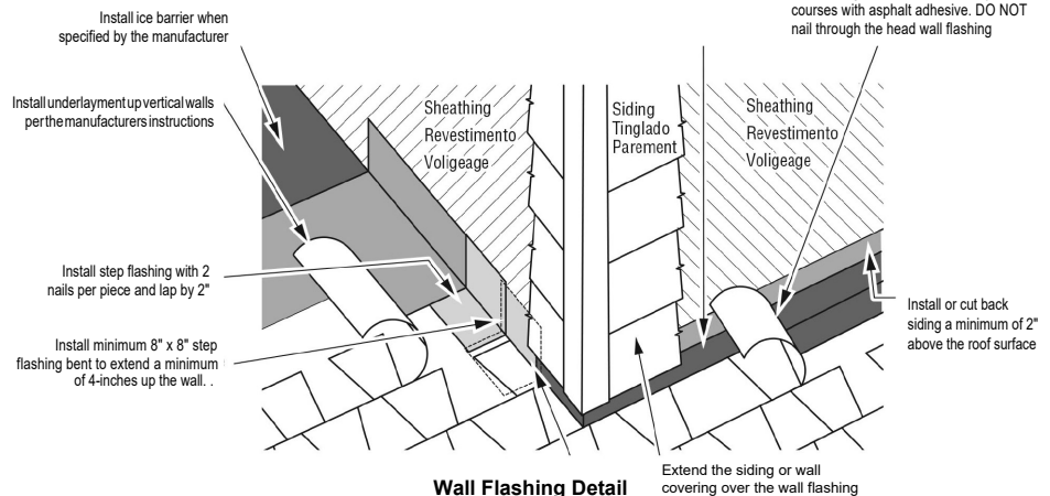
Wall Flashing Detail
