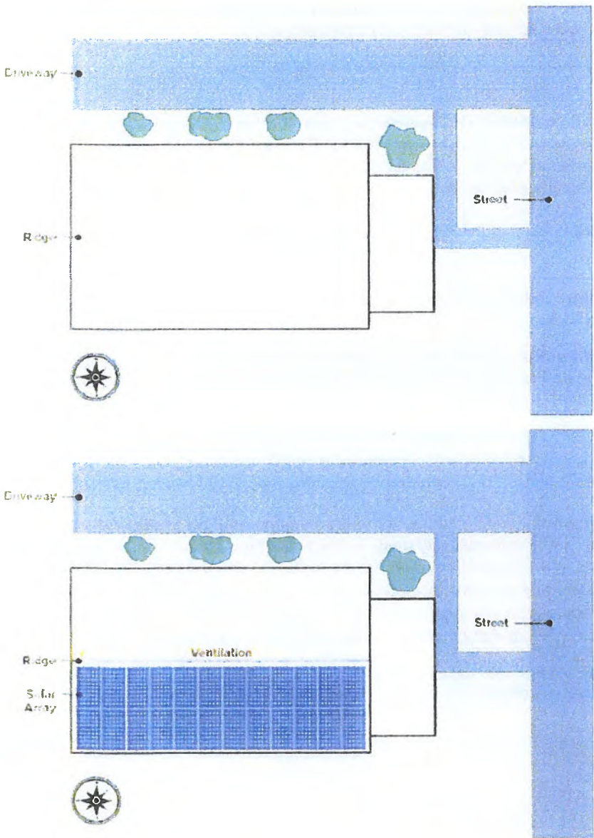
Typical single ridge roof with alternative ventilation (Figure 2)
